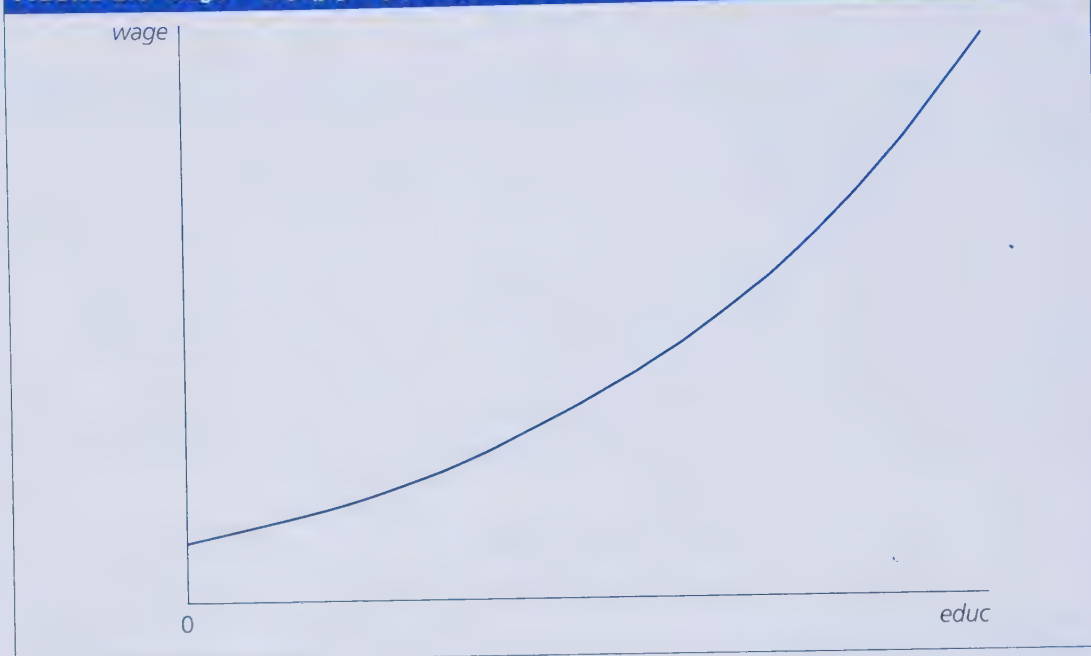
FIGURE 2.6 wage = \exp(\beta_0 + \beta_1 educ) , with \beta_1 > 0 .
