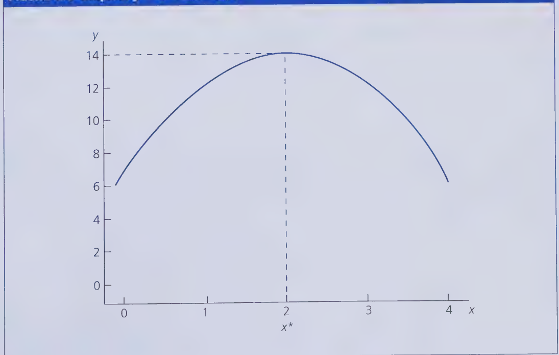
FIGURE A.3 Graph of y = 6 + 8x - 2x^2 .
