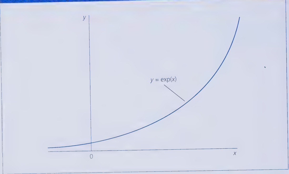
FIGURE A.5 Graph of y = \exp(x) .
