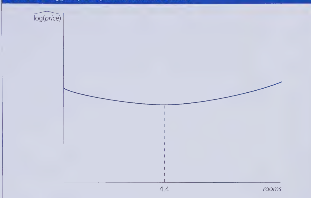
FIGURE 6.2 \widehat{\log(\text{price})} as a quadratic function of rooms .
