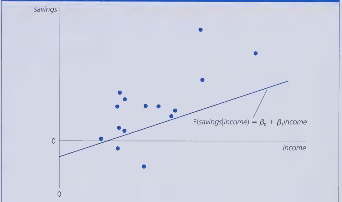
FIGURE 2.2 Scatterplot of savings and income for 15 families, and the population regression E(\text{savings}|\text{income}) = \beta_0 + \beta_1 \text{income} .
