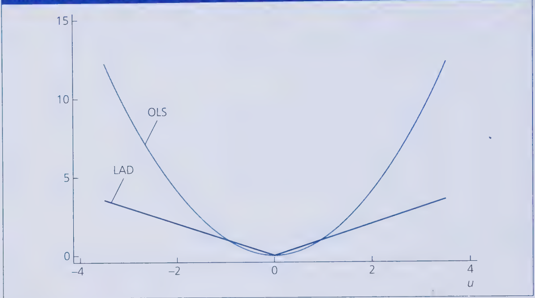
FIGURE 9.2 The OLS and LAD objective functions.
