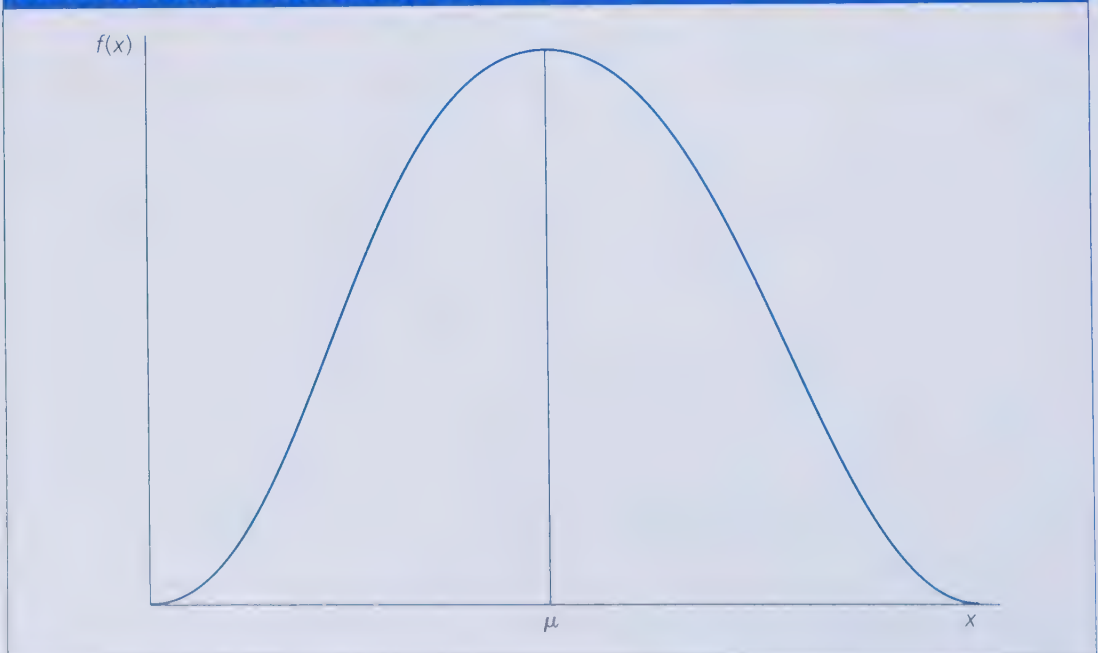
FIGURE B.3 A symmetric probability distribution.
