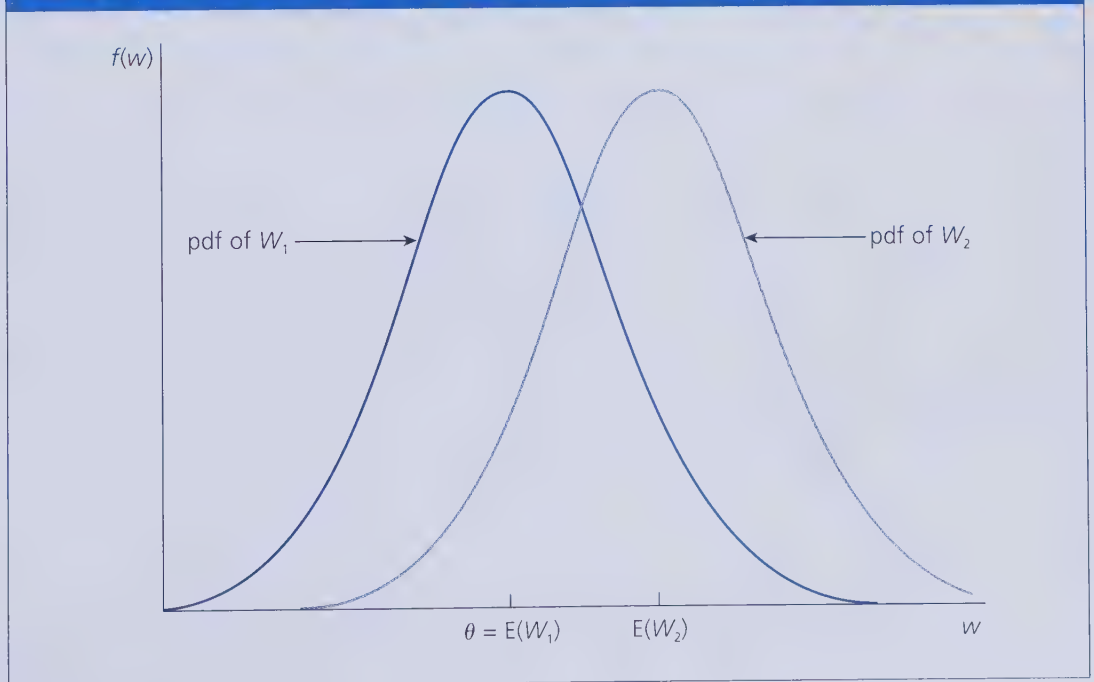
FIGURE C.1 An unbiased estimator, W_1 , and an estimator with positive bias, W_2 .
