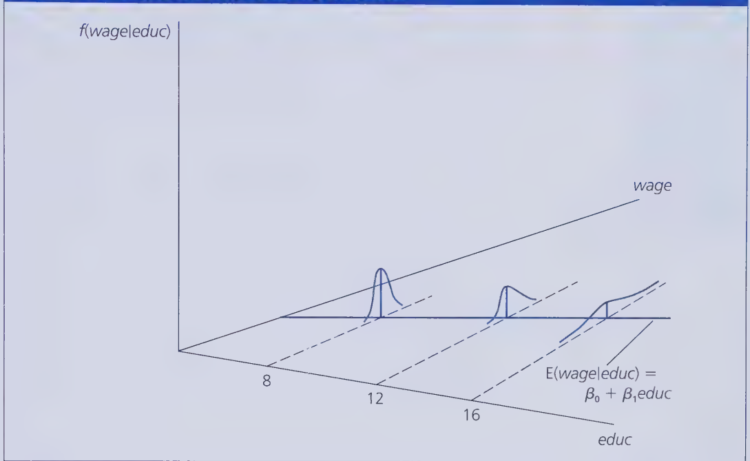
FIGURE 2.9 \text{Var}(\text{wage}|\text{educ}) increasing with \text{educ} .
