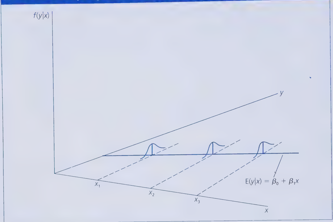
FIGURE 2.8 The simple regression model under homoskedasticity.
